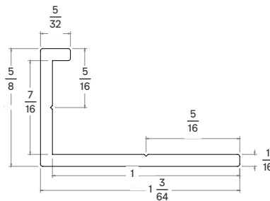
Type BM - 1/2"
