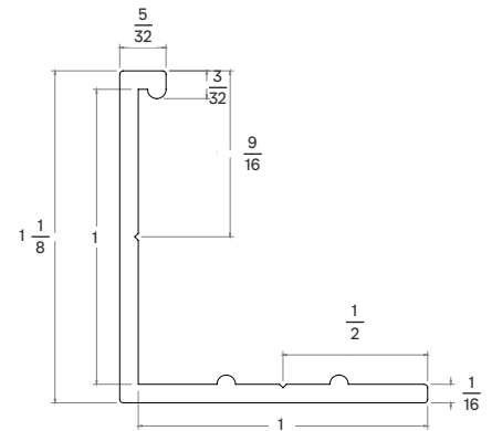
Type CM - 1"
