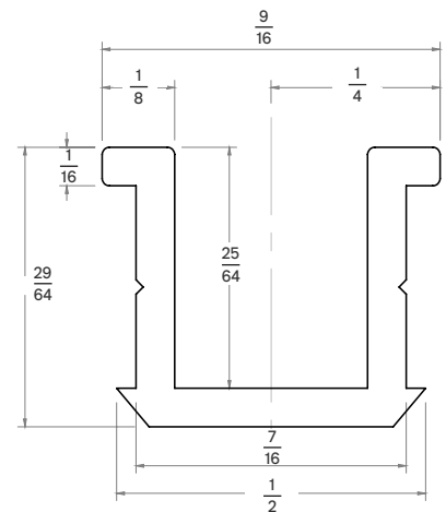
Type FM - 2"
