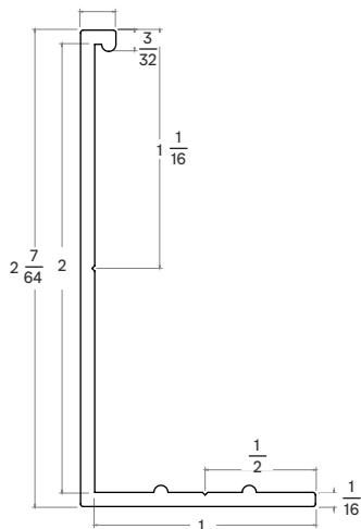
Type DM - 2"
