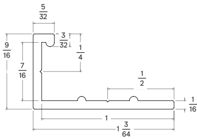
Type AM - 13/32"
