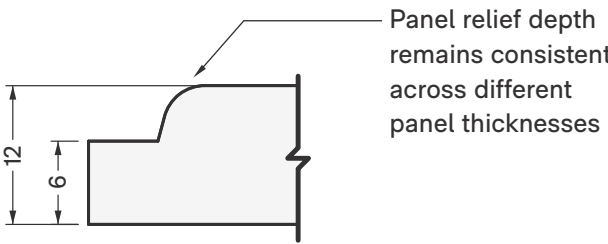
12mm Thickness (6mm Edge Thickness)
