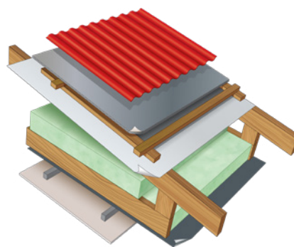
Roof with Steel Purlins
