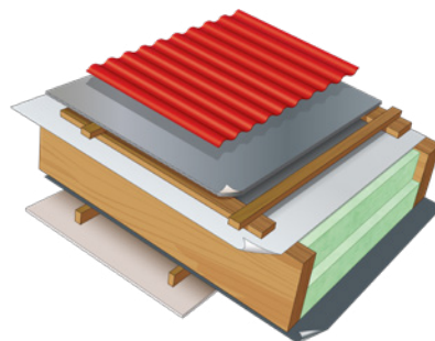
Trussed Roof
