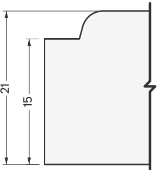
21mm Thickness (15mm Edge Thickness) Not available in Pinstripe
