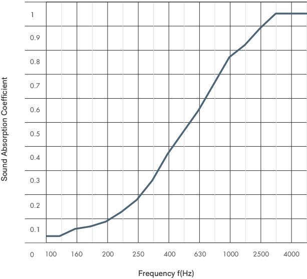
Absorption Coefficient According ISO 354 University of Auckland Testing Service Composition Peel 'n' Stick Tiles (0.4" - 0.5") - Test No. T0814-2b
