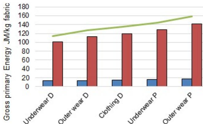
Figure 8. PET Fabric MJ/kg
