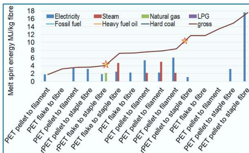
Figure 4. PET Melt-spin Gross Energy & Sources
