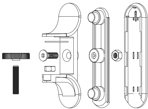
Exploded View
