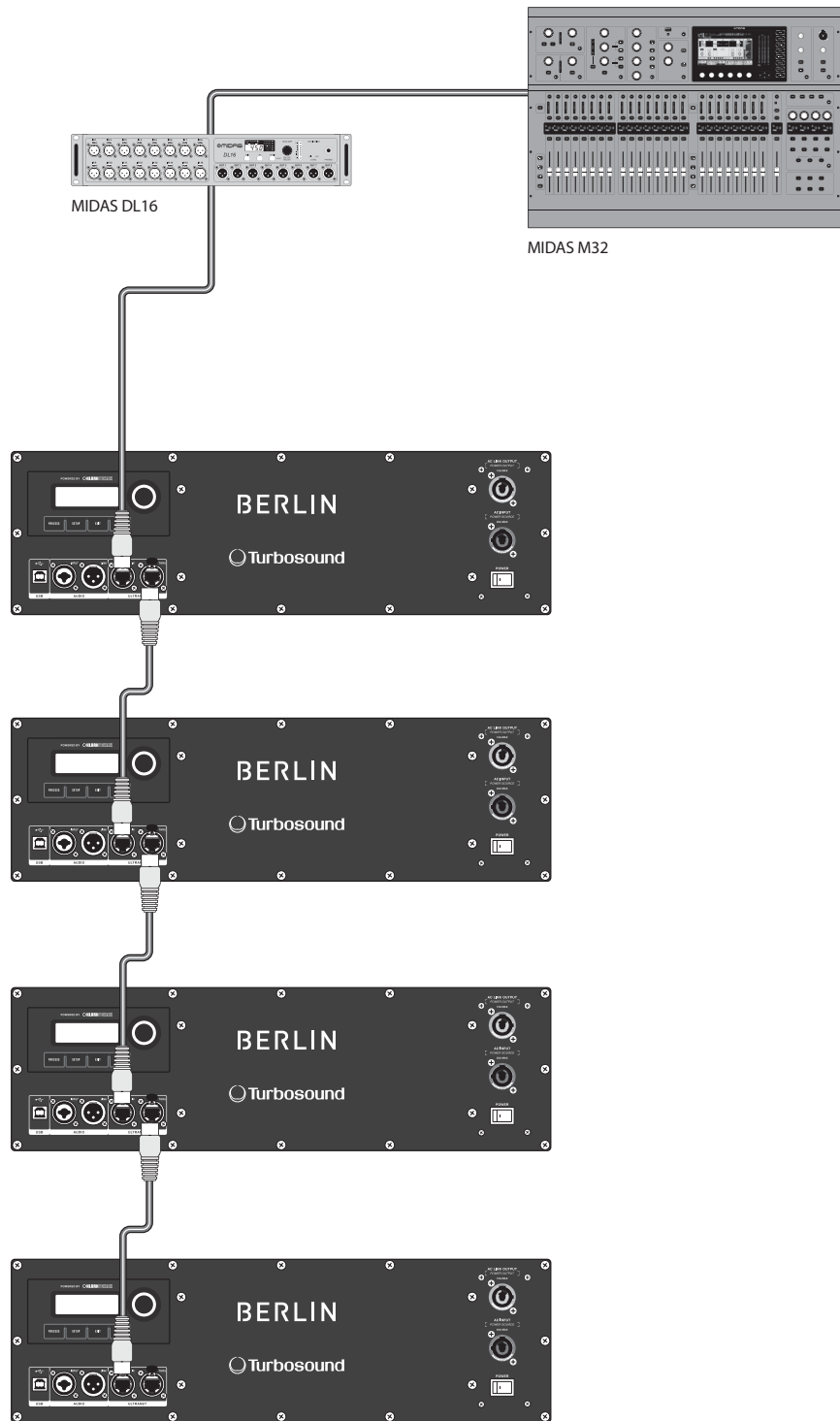
ULTRANET connection with MIDAS M32 digital mixer and MIDAS DL16 digital snake
