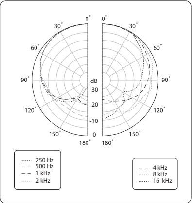
Polar pattern
