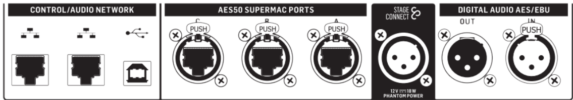
Figure 6: ETHERNET/AES50/Control/StageConnect connectors
