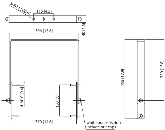
轭垂直 VX 12/VX 12.2 (-WH)
