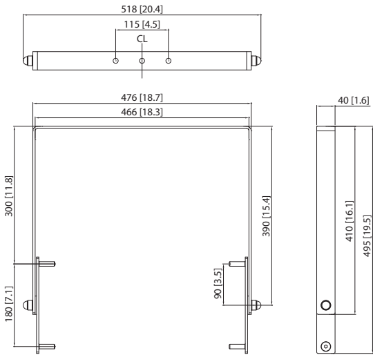
轭垂直 VX 12/VX 12.2 (-WH)
