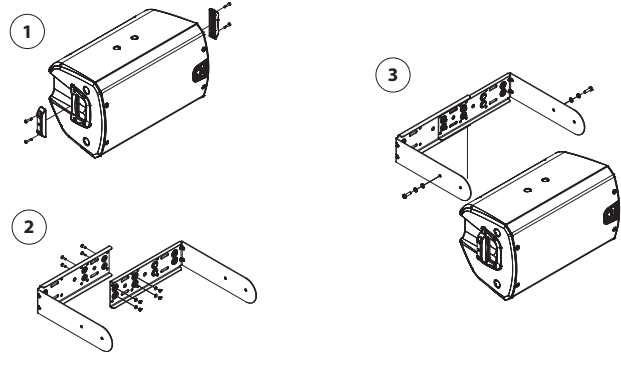
Step 1: Secure Yoke Spacers
