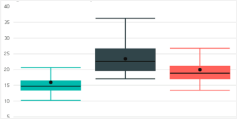
Dashboarding
