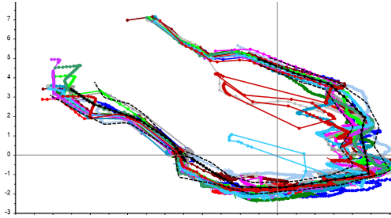
Data Analytics
