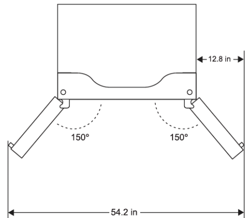
TOP OF REFRIGERATOR WITH DOORS OPEN 150°
