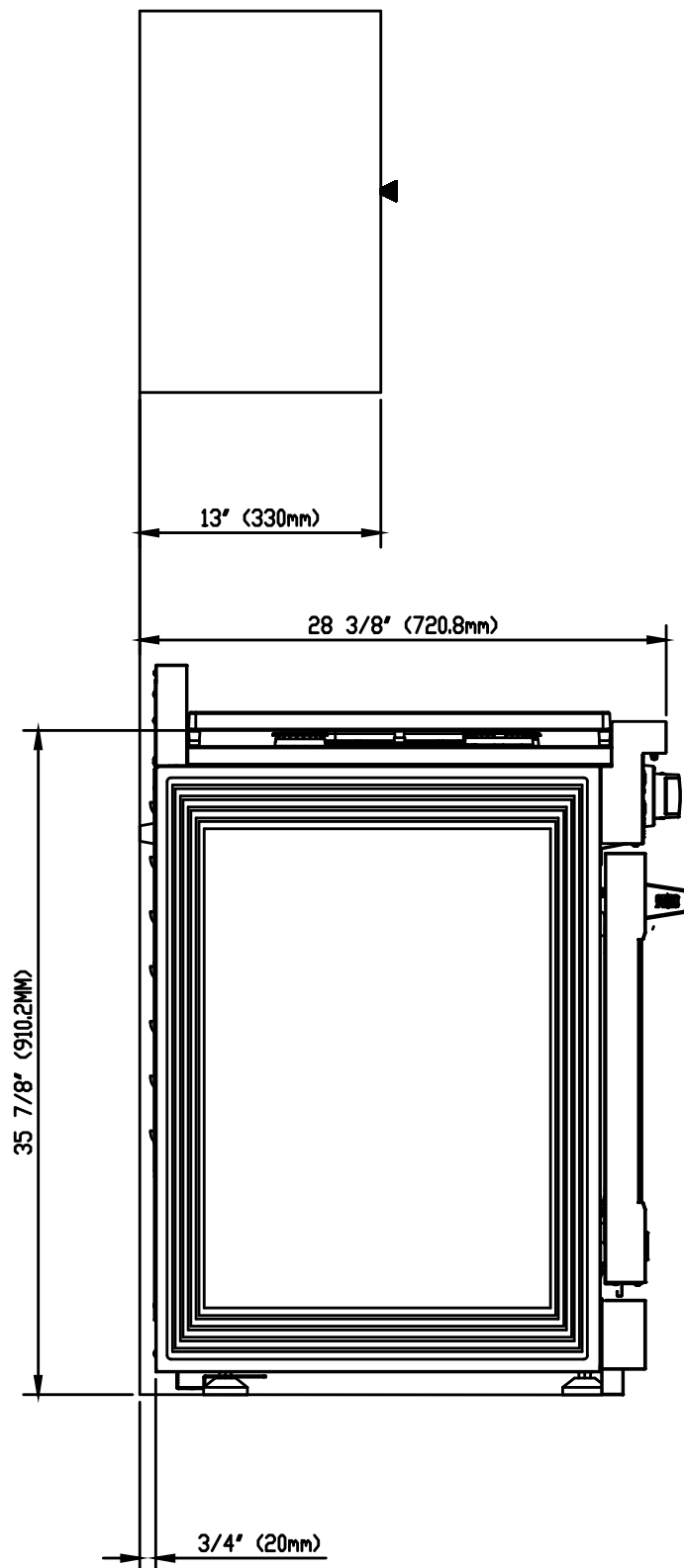
Side View
