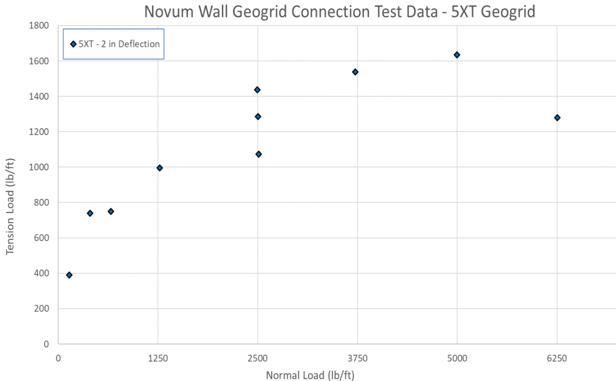
Figure 6 – Peak Connection Strength versus Normal Load
