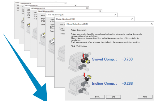
Guidance display when using 3-axis adjustment table
