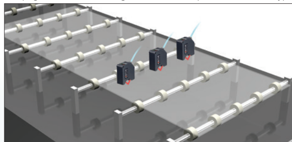
Warpage measurement of glass substrates (specular reflection type)
