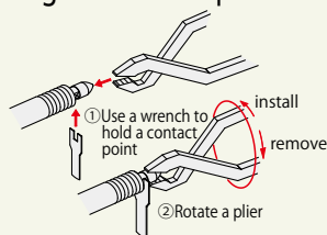
【How to install/remove the contact point】
