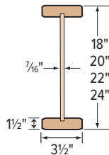
AJS 25 Joists
