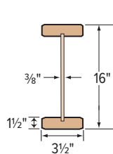
AJS 25 Joists
