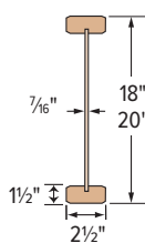
AJS 190 Joists
