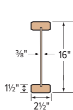
AJS 190 Joists
