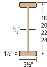
AJS 30 Joists
