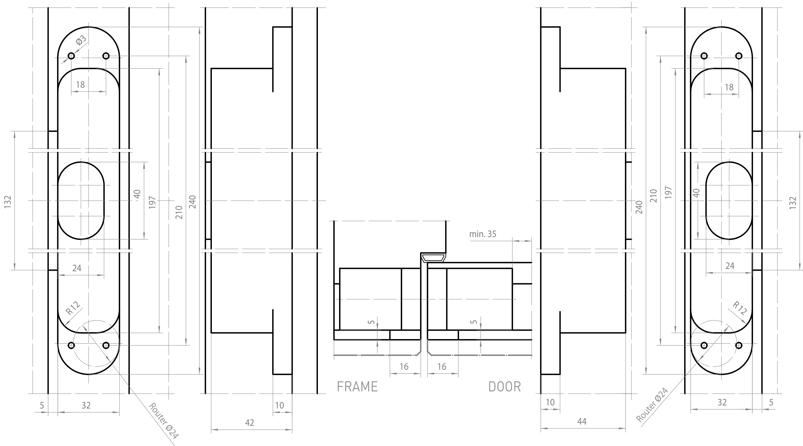
TE 640 3D A8 ENERGY : BLOCK FRAME TE 626 3D A8 ENERGY
