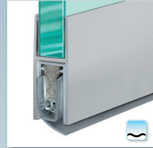
Option: Planet G-F12s | F16s, bevel lip for uneven floors
