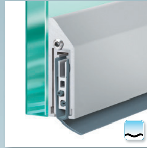
Option: Planet KG-S narrow, bevel lip for uneven floors
