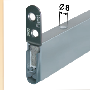
Option: Planet HS-plus with Planet drill hole \varnothing 8 mm for driving bar rods → refer to chapter Accessories | driving bar rods
