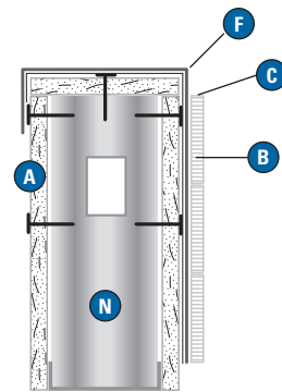
Knee wall details
