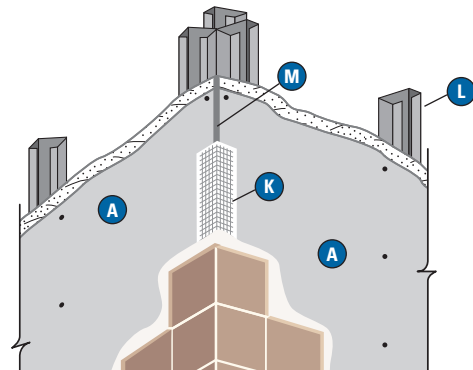
Corner detail with flexible sealant and joint finishing
