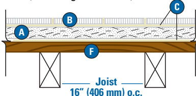
DensShield Tile Backer Over Conventional Joist (Exterior-glove Subfloor)
