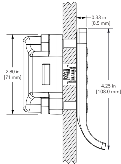
Side View-Cable
