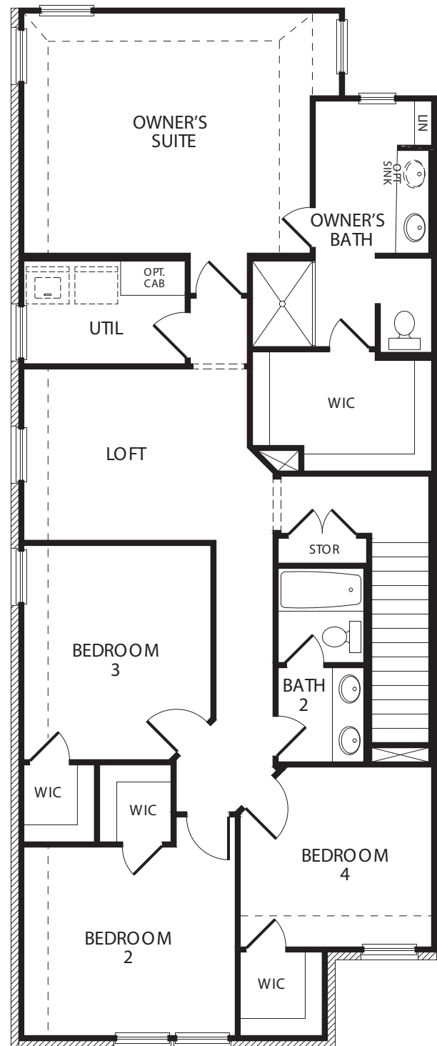
SECOND FLOOR
