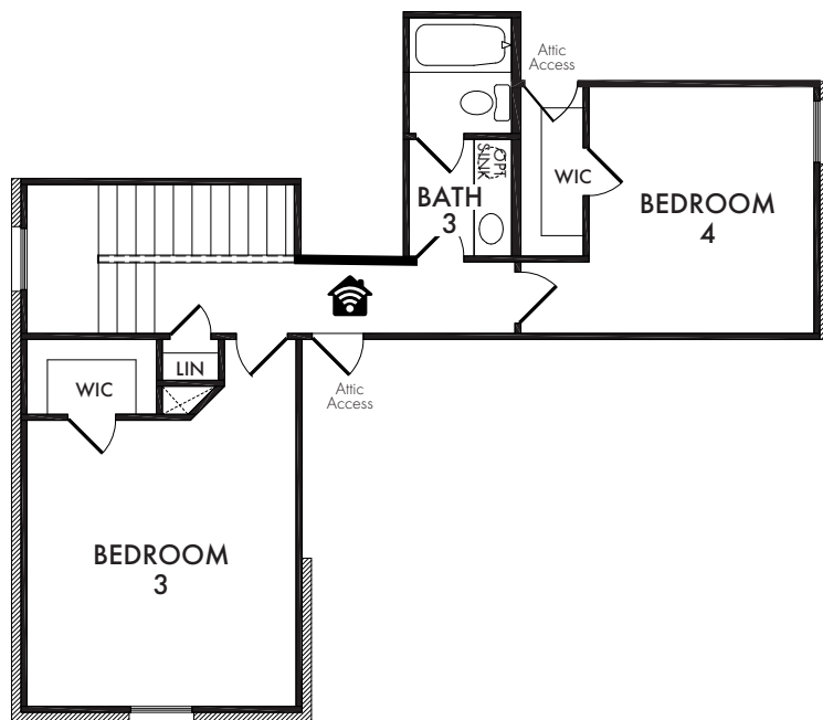
SECOND FLOOR
