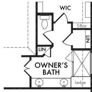
OPTIONAL OWNER'S BATH w/Shower Only
