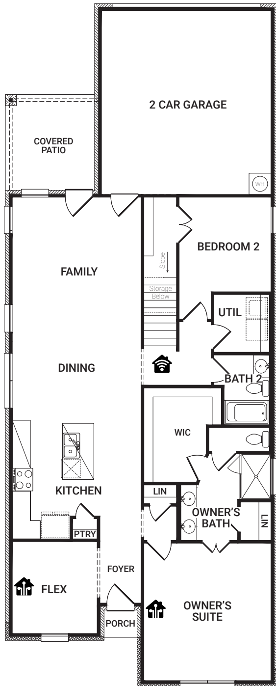
FIRST FLOOR
