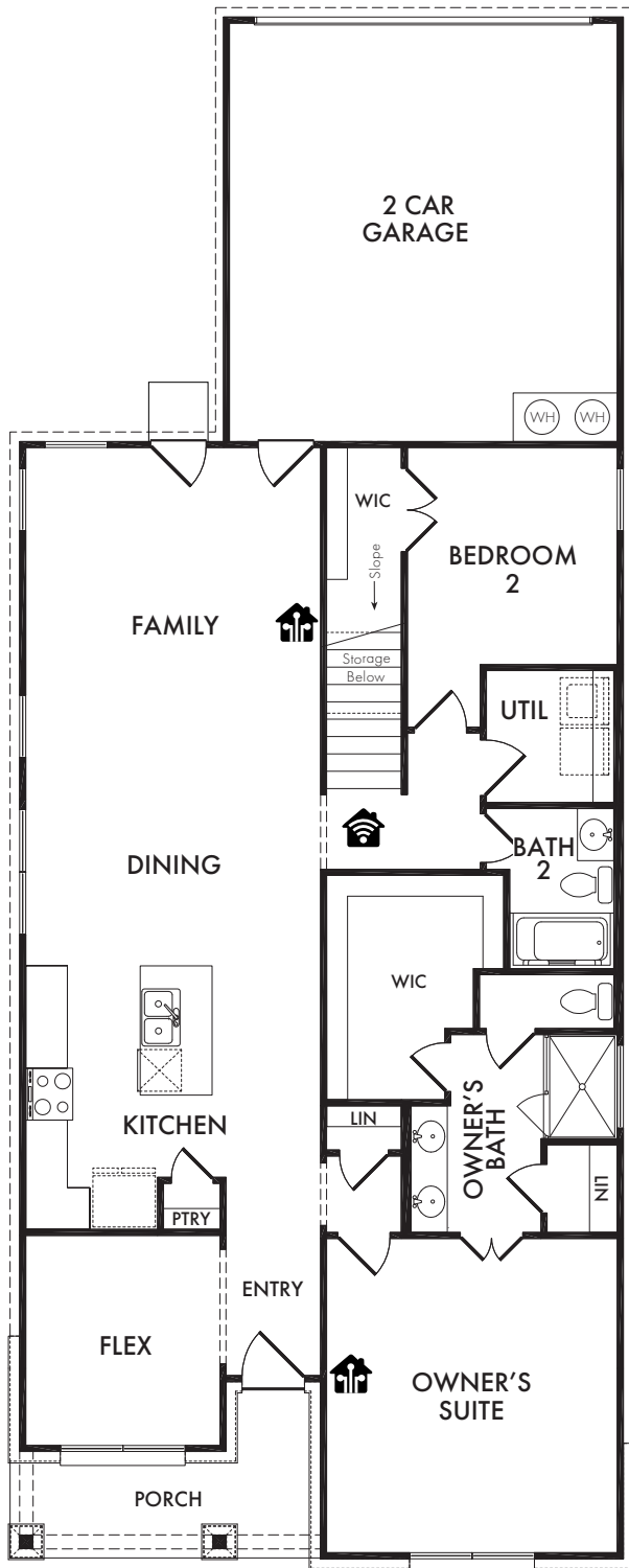
FIRST FLOOR
