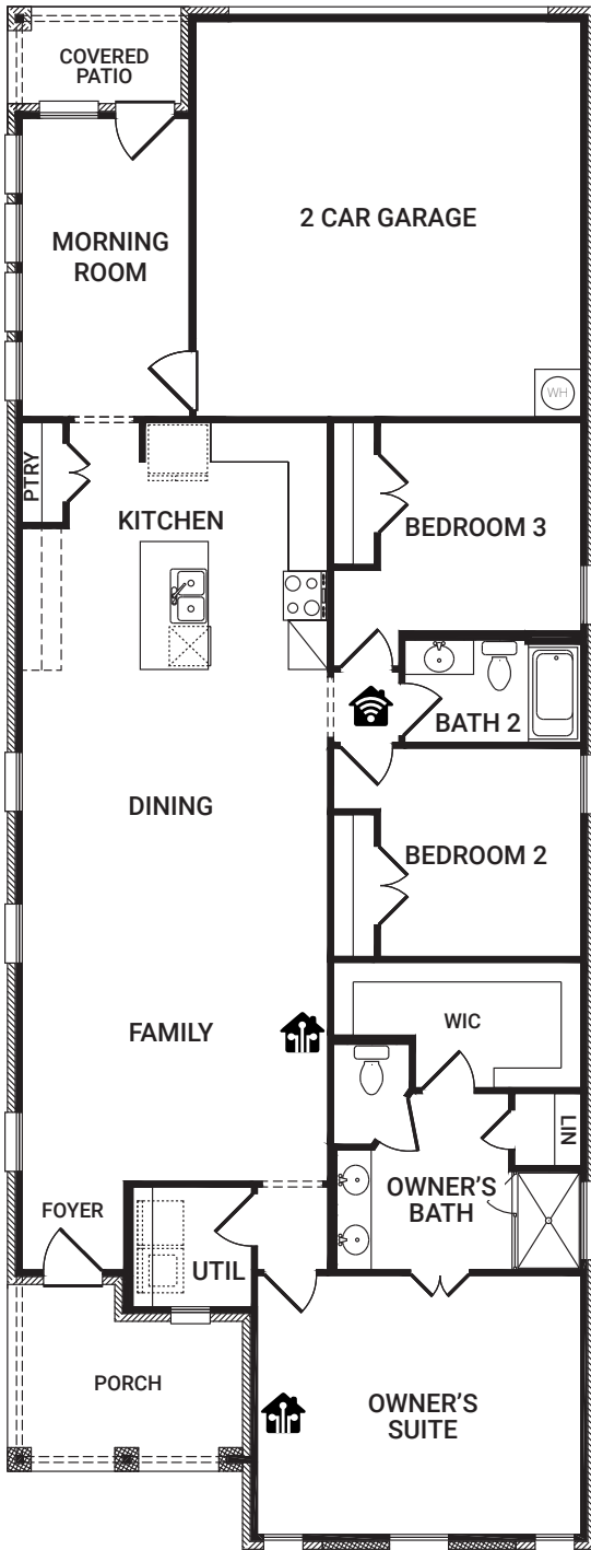
OPTIONAL OWNER'S BATH Half Wall OPTION #202
