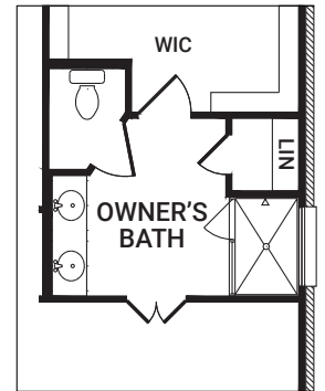
OPTIONAL OWNER'S BATH 2nd Vanity Bowl Included Standard OPTION #206
