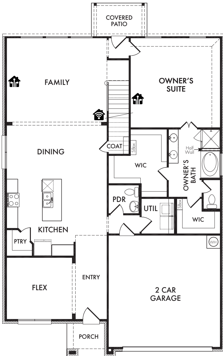
FIRST FLOOR
