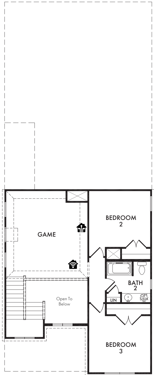
SECOND FLOOR
