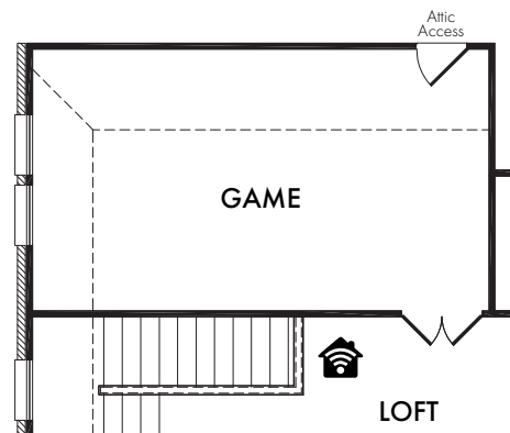
OPTIONAL GAME ROOM (Adds Approx. 315 Sq. Ft.)
