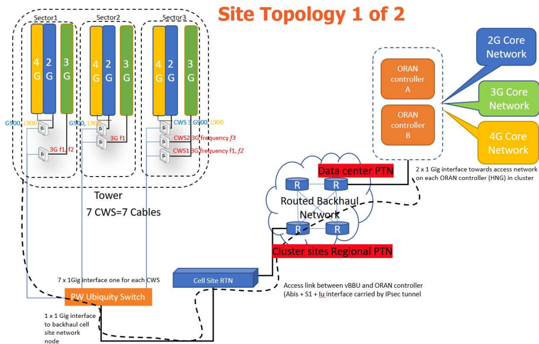
Figure 14 – trial site topology
