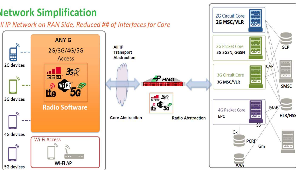
Figure 9 – Parallel Wireless solution architecture
