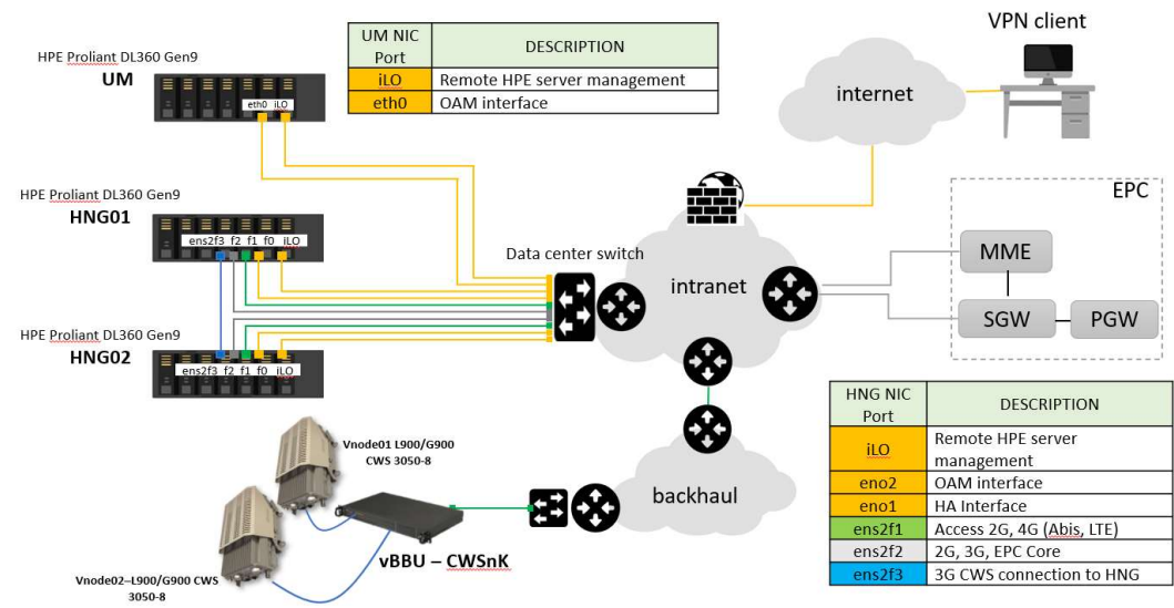
Figure 11 – Vodafone Turkey GSM/LTE multi-RAT network solution
