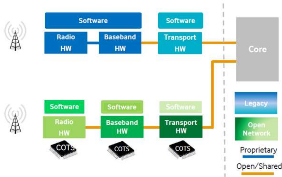
Figure 1 –Architecture Overview
