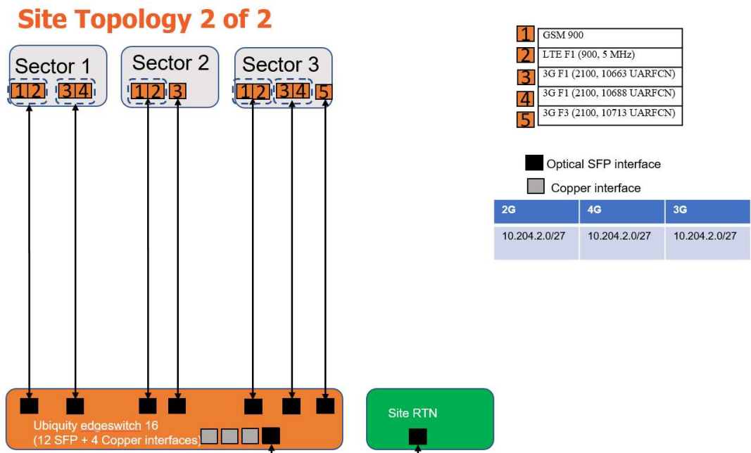
Figure 15 – Dodurga trial site topology
