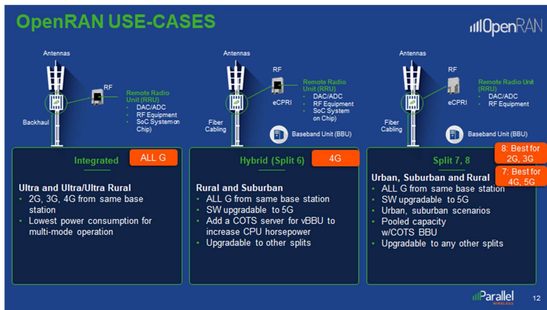
Figure 16 – Supported types of OpenRAN use cases
