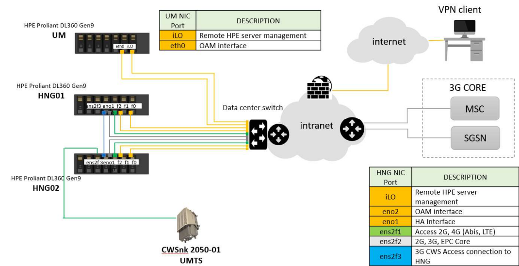
Figure 12 – Vodafone Turkey 3G ATP network solution
