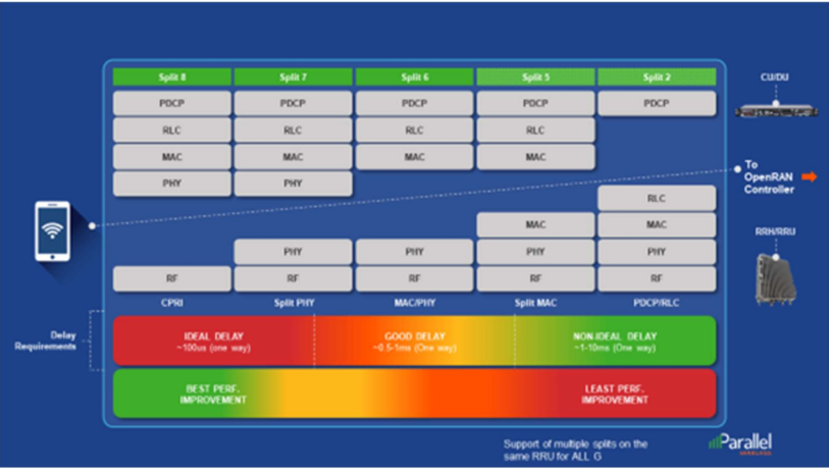
Figure 17 – RAN Split options overview
